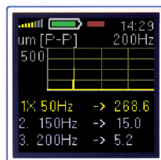
FFT Spectrum
